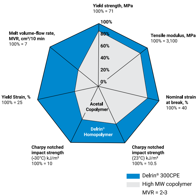
Figure 6. Comparison of Delrin® 300CPE homopolymer vs. high molecular weight standard acetal copolymer
