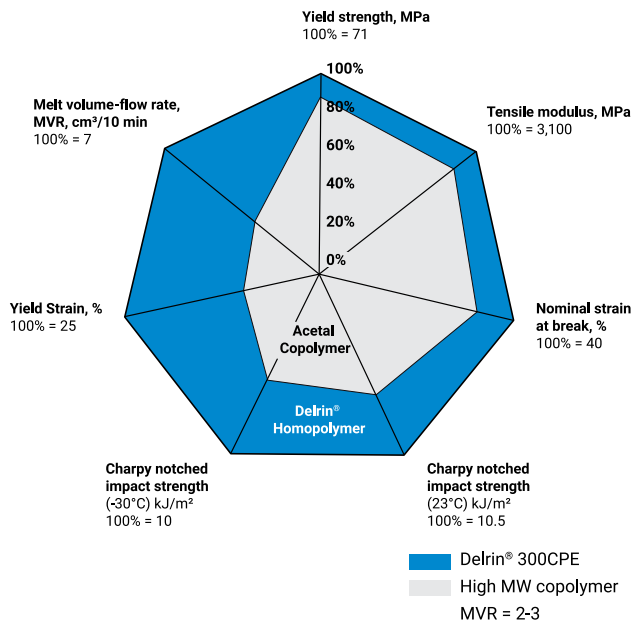
Figure 7. Comparison of Delrin® 100CPE homopolymer vs. high molecular weight standard acetal copolymer
