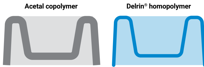
Figure 11. The superior mechanical properties of Delrin® homopolymer can allow thinner wall sections compared to acetal copolymers for the same physical part capabilities
