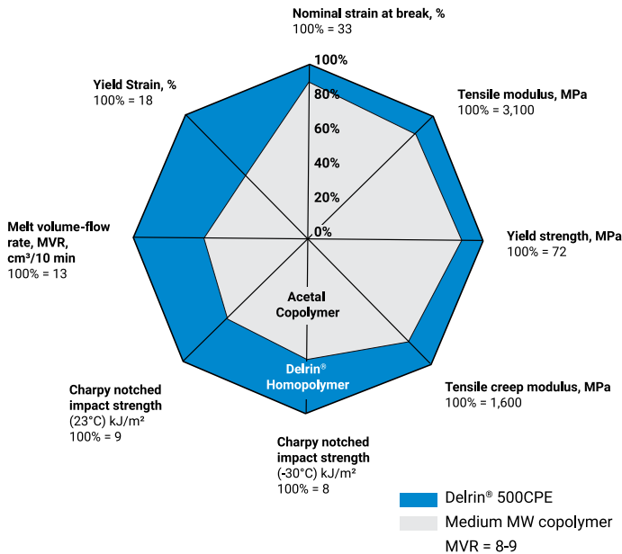
Figure 5. Comparison of Delrin® 500CPE homopolymer vs. general purpose acetal copolymer
