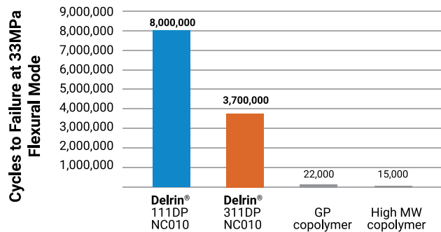
Figure 9. Comparison of resistance to flexural fatigue at 33MPa loading of various Delrin® homopolymer grades vs. standard acetal copolymer grades
