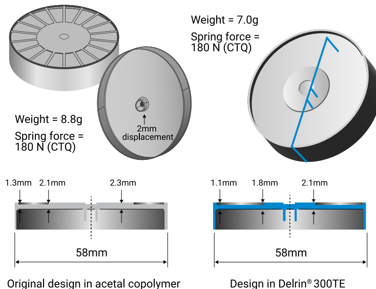
Figure 10. Original design based on acetal copolymer vs. optimized design using Delrin® homopolymer
