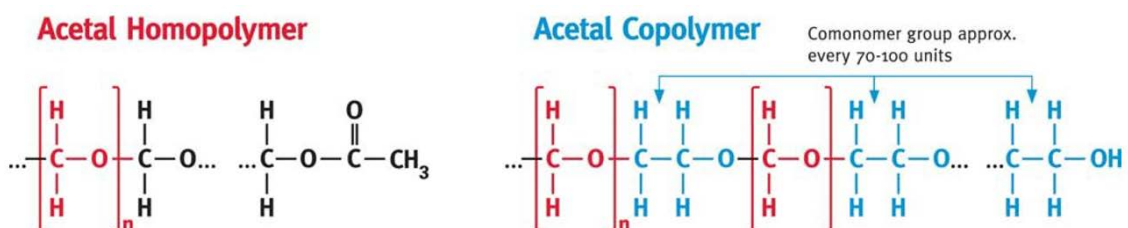
Figure 1. Molecular structure of acetals
