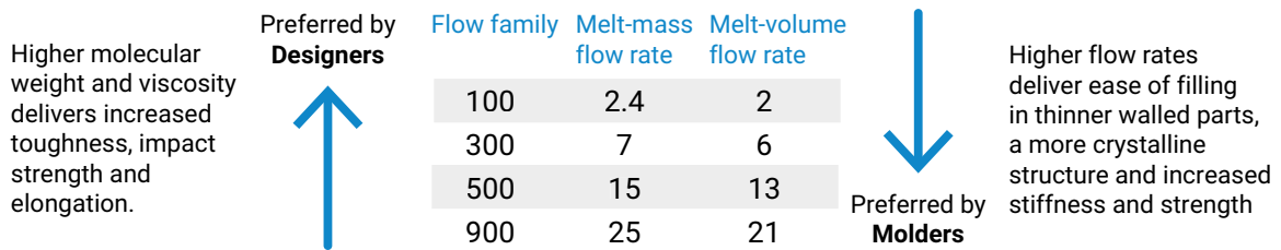
Figure 3. Property trends with changes in flow family
