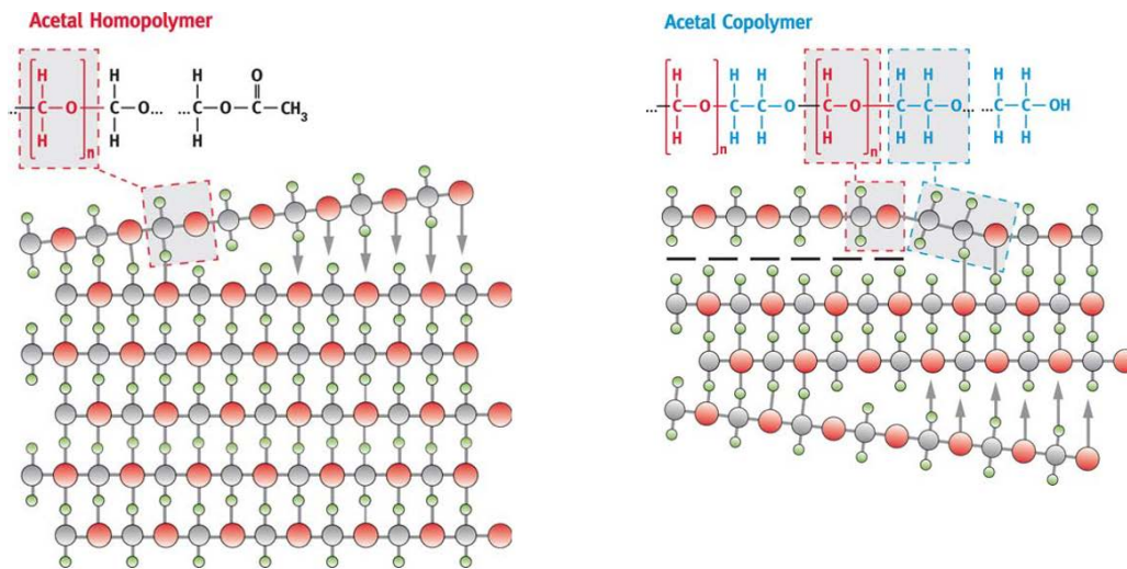
Figure 2. Delrin® homopolymer vs. acetal copolymer crystalline structure in 2-D
